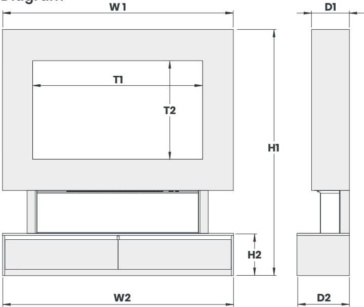
Dimensions - DEEP
