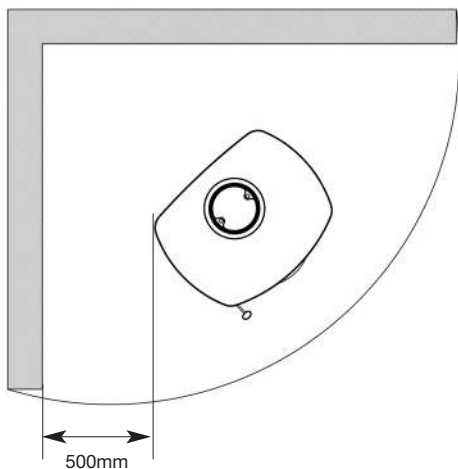
Neo corner installation, insulated / single skin flue with / without heat shield.
